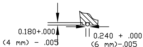
GROOVE DETAIL
