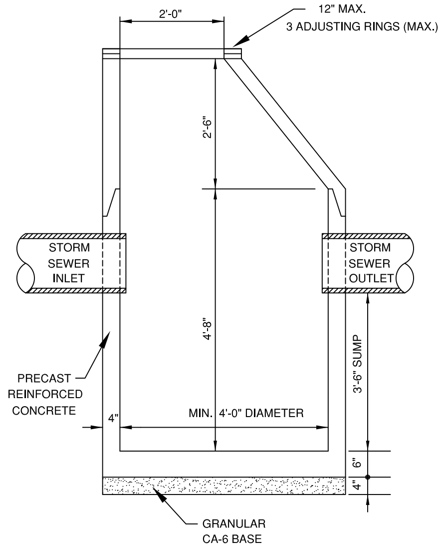
CATCH BASIN (TYPE A)
