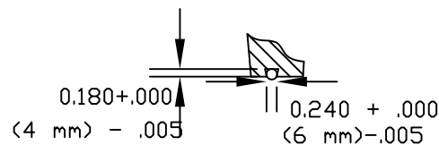
GROOVE DETAIL
