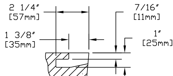
PICK HOLE DETAIL
